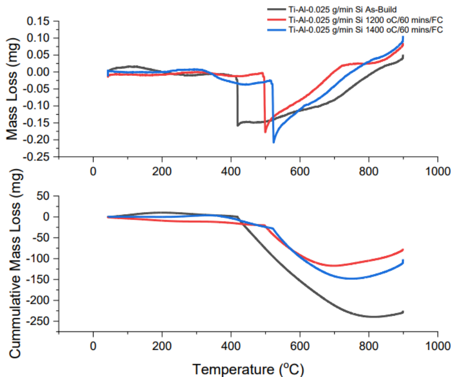
Figure 4: TGA Curves of Ti-Al-0.025 g/min Si Alloy
