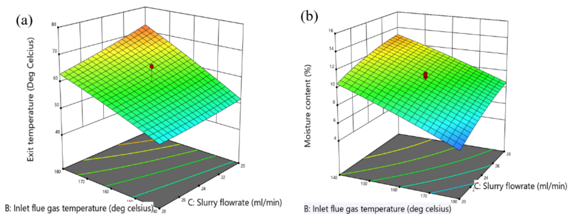
Figure 7: 3D surface graphs of the influence of inlet flue gas temperature and slurry flowrate on (a) exit temperature and (b) moisture content.
