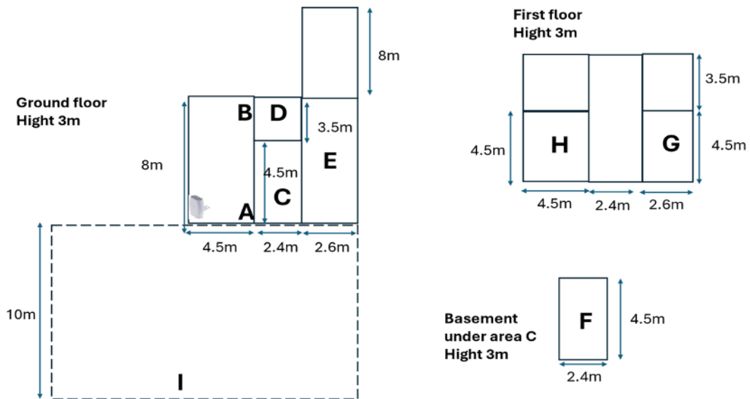
Figure 5: Experimental Setup- the gateway is placed on the ground floor. The letters A-I denote the position of LoRaWAN end-device.
