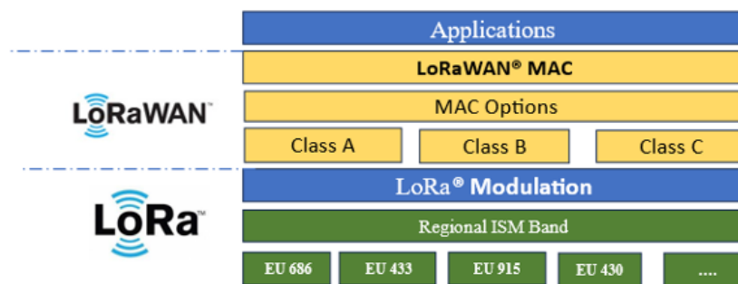
Figure 3: LoRa and LoRaWAN OSI model
