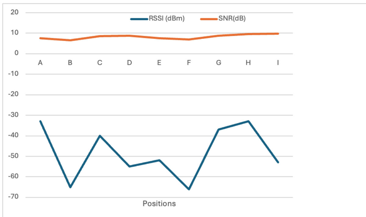
Figure 6: The LoRaWAN coverage measurements and results
